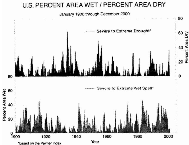
FIG. 6. The percent area of the contiguous United States experiencing monthly (top) severe to extreme long-term drought and (bottom) severe to extreme long-term wet conditions during the twentieth century, based on the PMDI. The major (national scale) drought episodes stand out, with drought reaching its greatest extent during the “dust bowl” years of the 1930s. At its peak, drought covered 63% of the nation during Jul 1934, with a secondary peak of about 43% during Aug 1936. The 1950s was another decade of drought, peaking at about 50% in Sep 1954 and 43% in Dec 1956. While significant droughts occurred in the 1980s and 1990s, severe to extreme wet spells were more prevalent. Similar time series could be created for other combinations of wet and dry Palmer categories.
