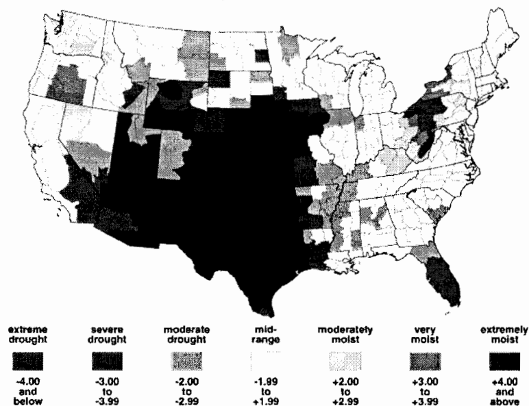
FIG. 5. The PMDI showing the cumulative long-term drought conditions for Sep 1956. During this month just under 40% of the contiguous United States experienced severe to extreme drought.
