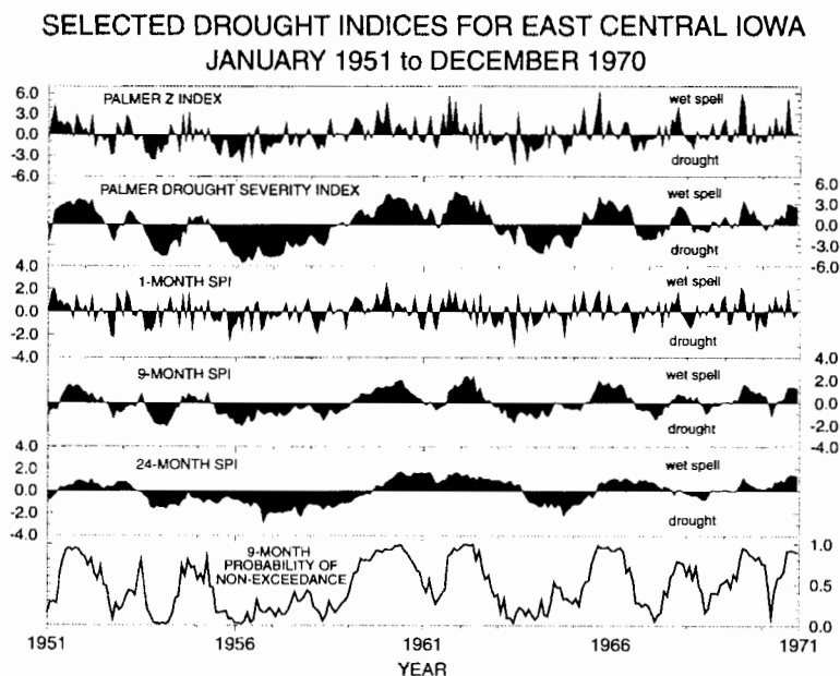
FIG. 7. Comparison of two monthly Palmer indices (the Z Index and the PDSI) to several SPI products for east-central Iowa for 1 Jan 1951–31 Dec 1970. Both the 1-month SPI and the Palmer Z Index measure short-term (i.e., monthly) drought. The 9-month SPI corresponds approximately to the PDSI. The versatility of the SPI is illustrated here by its ability to chart longer-scale drought (24-month SPI) and to put precipitation deficits into a probabilistic perspective. The utility of the particular index used depends on the application and what the user is trying to show. One cannot make a blanket statement that a particular index is better, overall, than another index.
