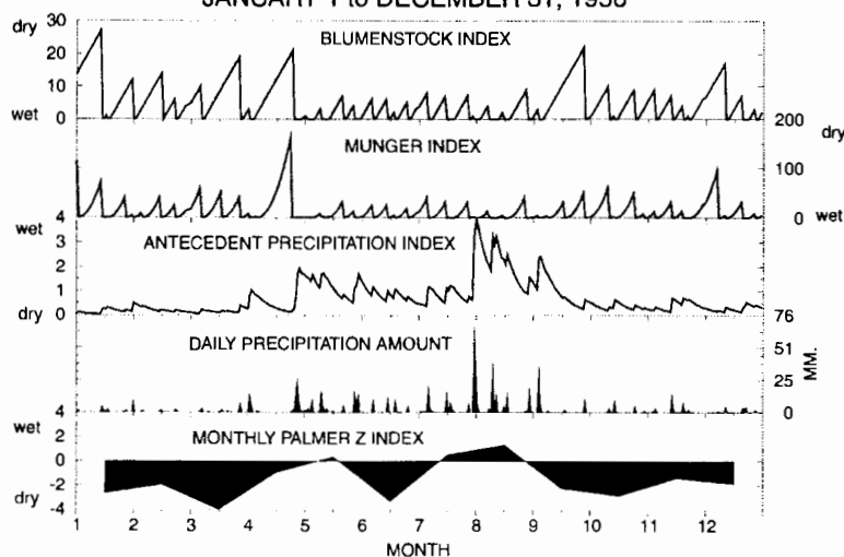
Fig. 1. Comparison of daily precipitation amount, three daily drought indices (the Blumenstock and Munger Indices and the API), and the monthly Palmer Z Index for east-central Iowa for 1 Jan–31 Dec 1956. Both the Blumenstock (1942) and Munger (1916) Indices are based on the length of the drought (in days), while the API (McQuigg 1954; Waggoner and O'Connell 1956) incorporated both the amount and timing of precipitation for flood forecasting and is, thus, a reverse drought index. These three indices are best suited for use on a short (daily to multimonthly) timescale.
