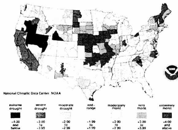
Palmer Drought Severity Index August, 2008
