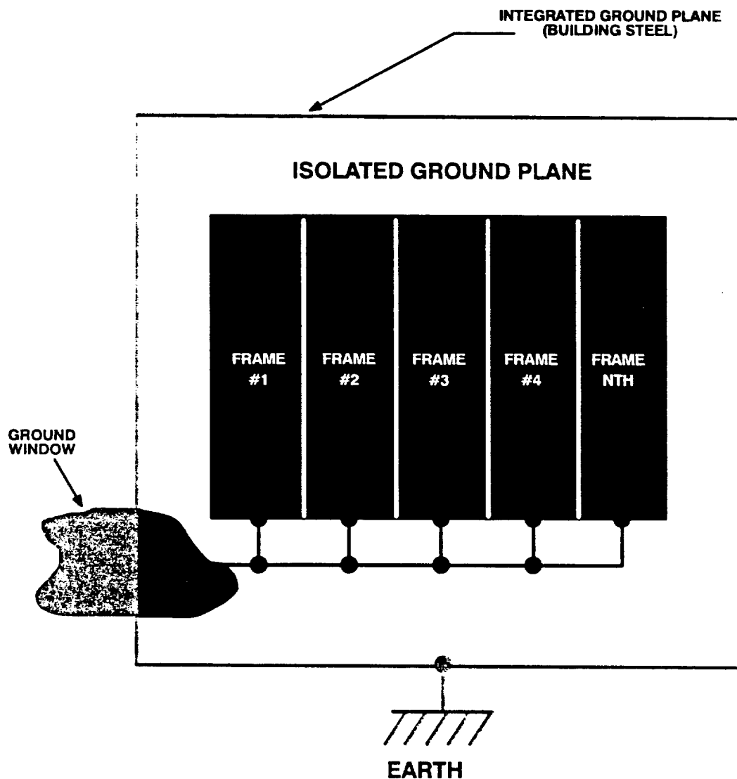
Figure 4-1. Simplified Isolated Ground Plane
